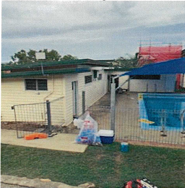
Photo ;2: Post removal soffits sheets
